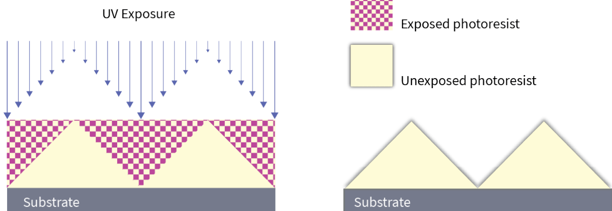
Figure 1: Schematic illustration of grayscale lithography. The photoresist layer is partially exposed by UV-light (left). During development, exposed resist is removed (right), resulting in a 2.5-dimensional topography.
